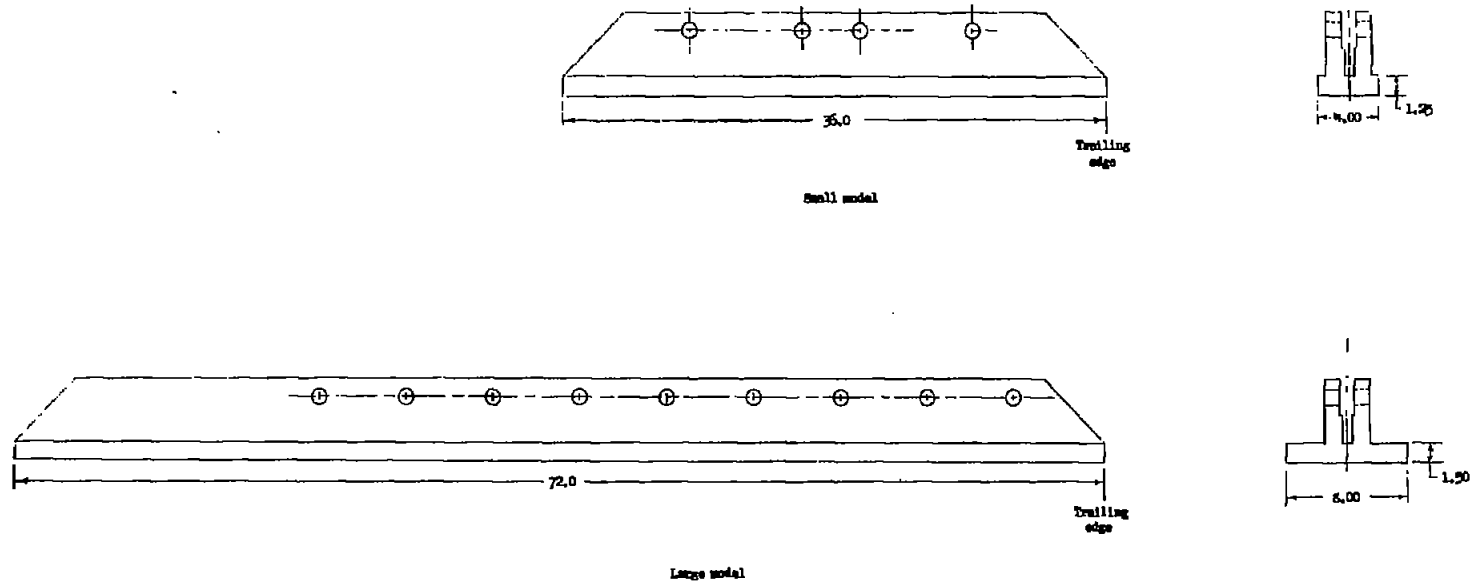
Figure 2.- Details of models. All dimensions are in inches.
