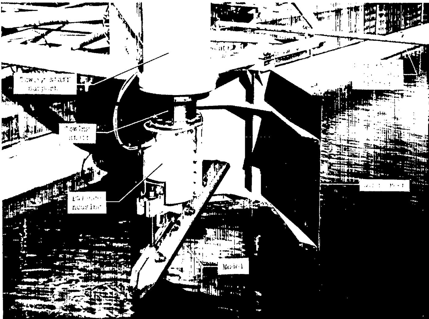
Figure 6.- Photograph of test setup with 4-inch-beam model installed.
