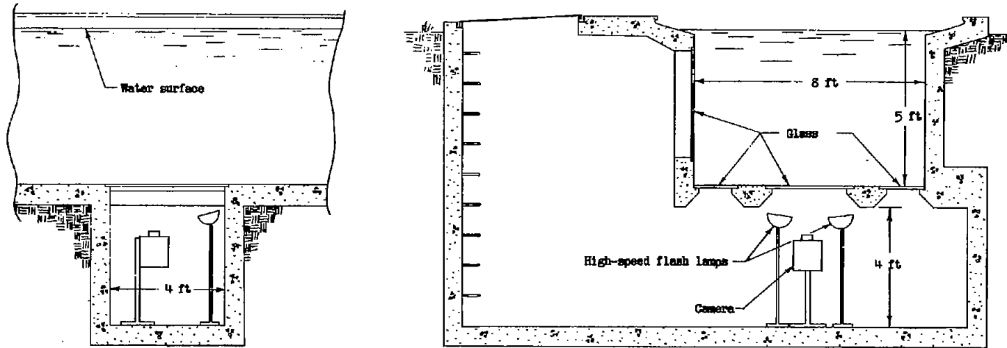
(a) Longitudinal cross section.
