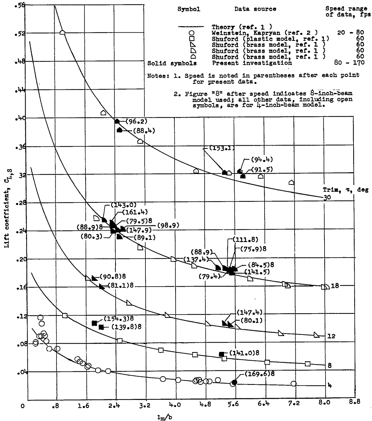
Figure 8.- Comparison of data from the high-speed hydrodynamics facility with theory and with data from lower speed towing tanks.
