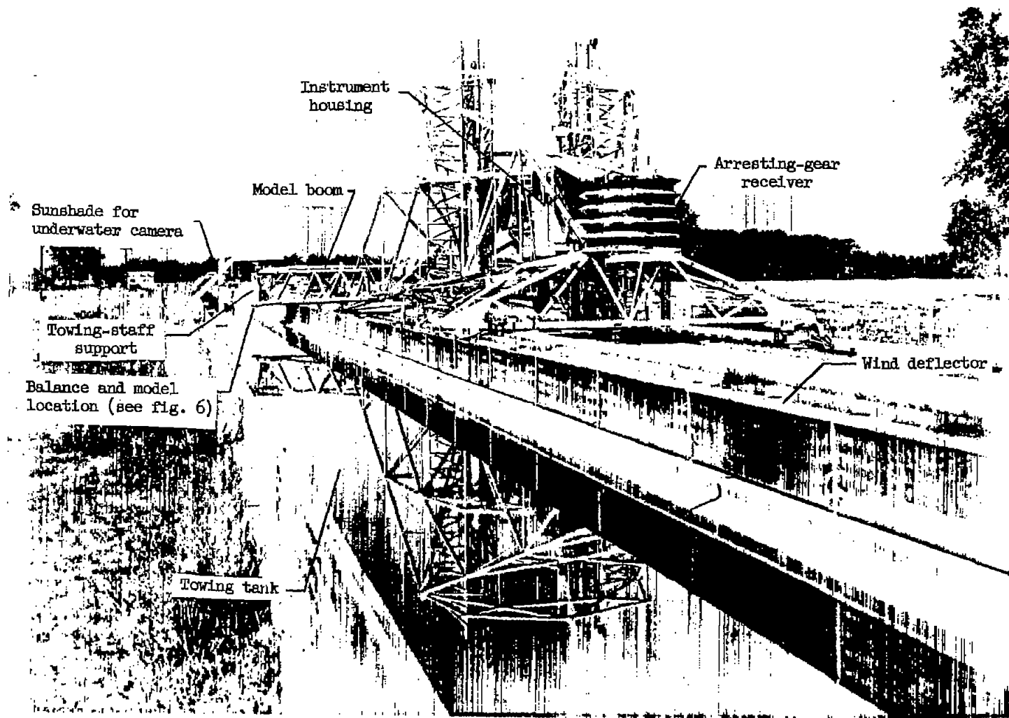
Figure 4.- Photograph of landing-loads carriage with temporary boom installed.
